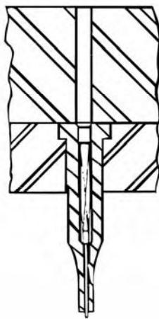
COMMON PIERCE PUNCH
