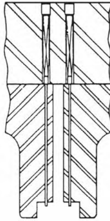
HEELED NOTCHING PUNCHES
