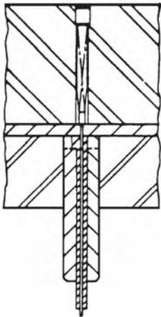
NARROW PUNCH IN SPLIT QUILL
