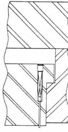
KNOCK-OUT IN COMPOUND DIE
